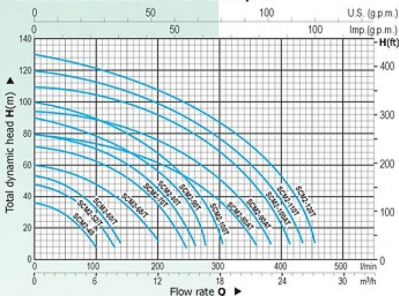
PERFORMANCE CHART AT n=2850r/min
